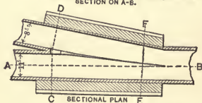
FIG. 6. JUNCTION OF 8 FT. AND 11 FT. SEWERS.
